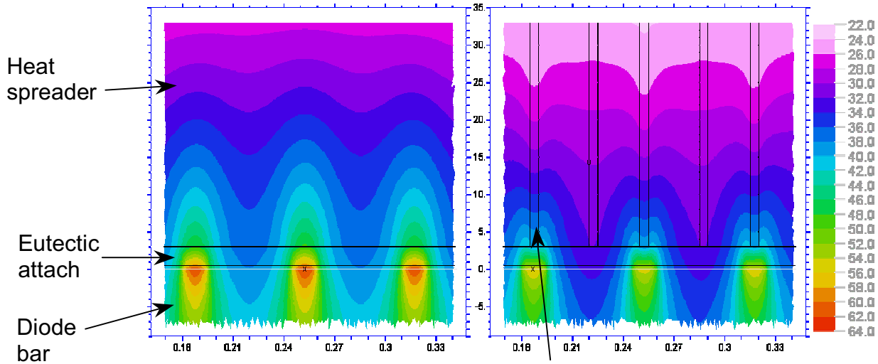
Polara heat spreader with Thermal Raceways added above emitters
