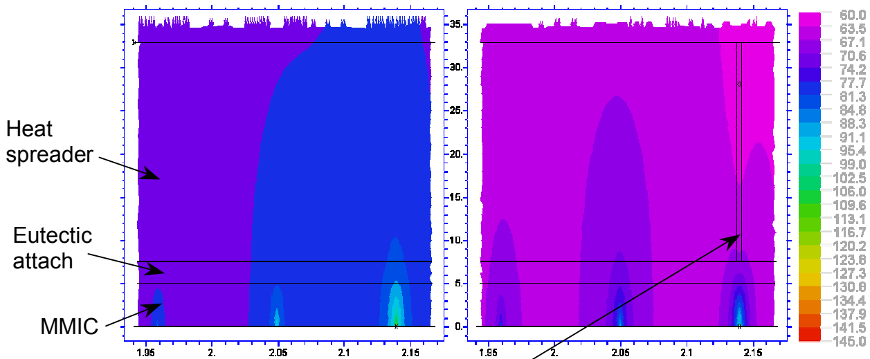
MMIC with Cu-Mo heat spreader
